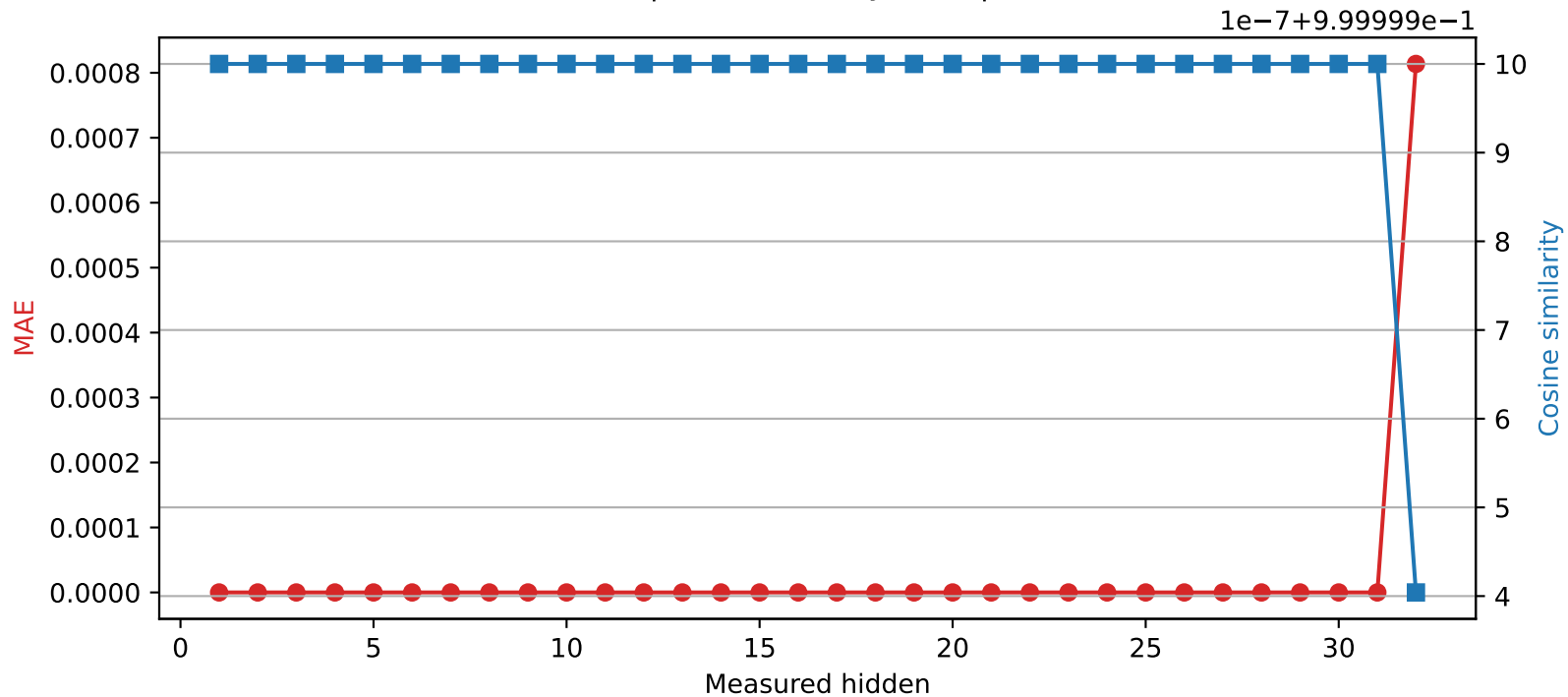
SmolLM2-360M | Quantized layer 31 | float64 → int16
