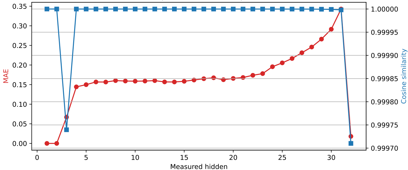
SmolLM2-360M | Quantized layer 2 | float16 \rightarrow int8
