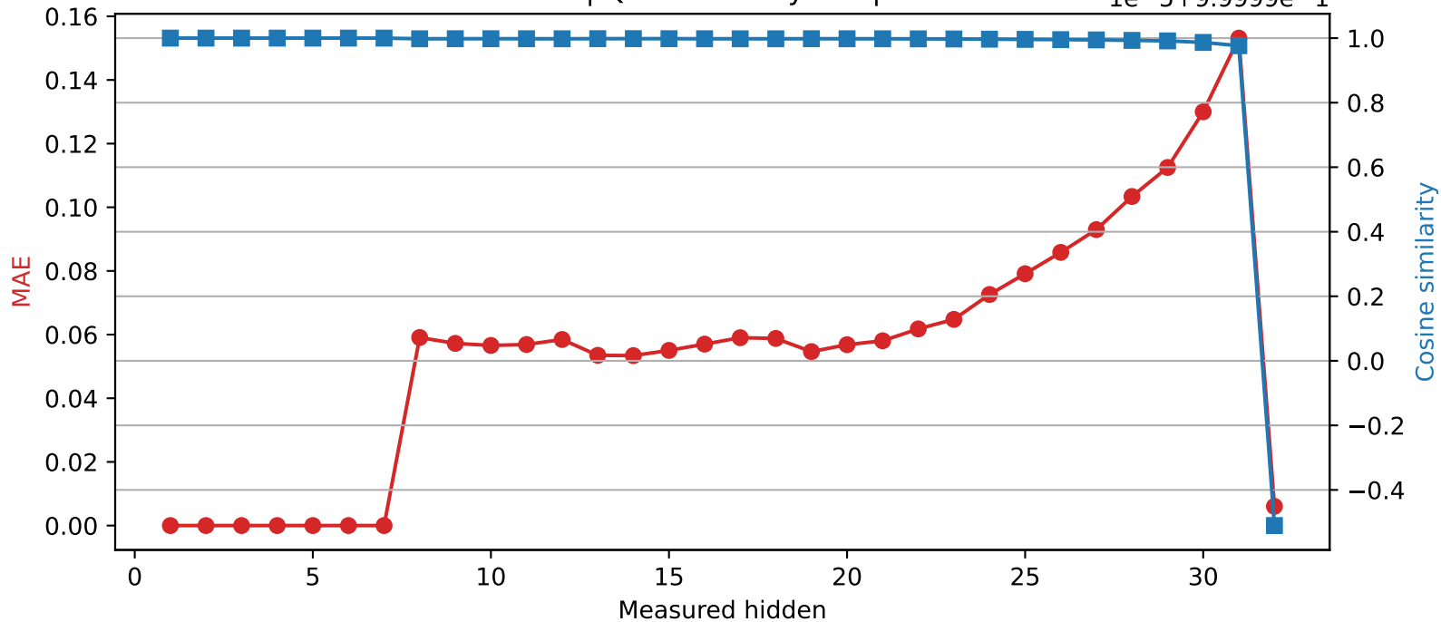
SmolLM2-360M | Quantized layer 7 | float16 \rightarrow int8 1e-5+9.9999e-1
