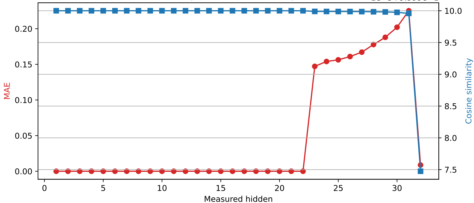
SmolLM2-360M | Quantized layer 22 | float16 → int8 1e-5+9.999e-1
