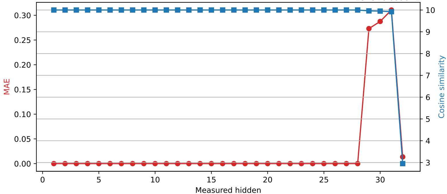
SmolLM2-360M | Quantized layer 28 | float16 \rightarrow int8 1e-5+9.999e-1
