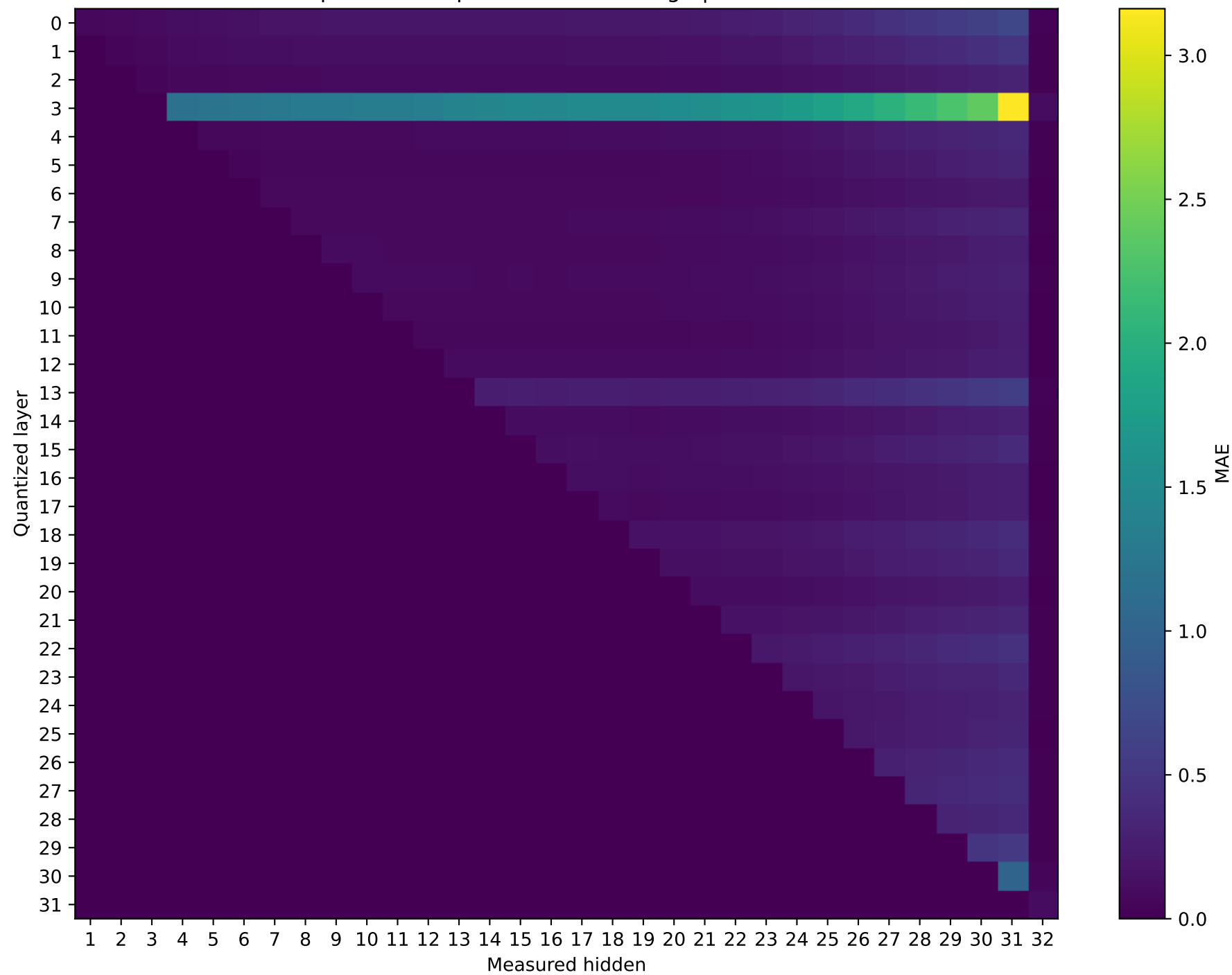
SmolLM2-360M Prompt 1: MAE representation damage | float16 → int8
