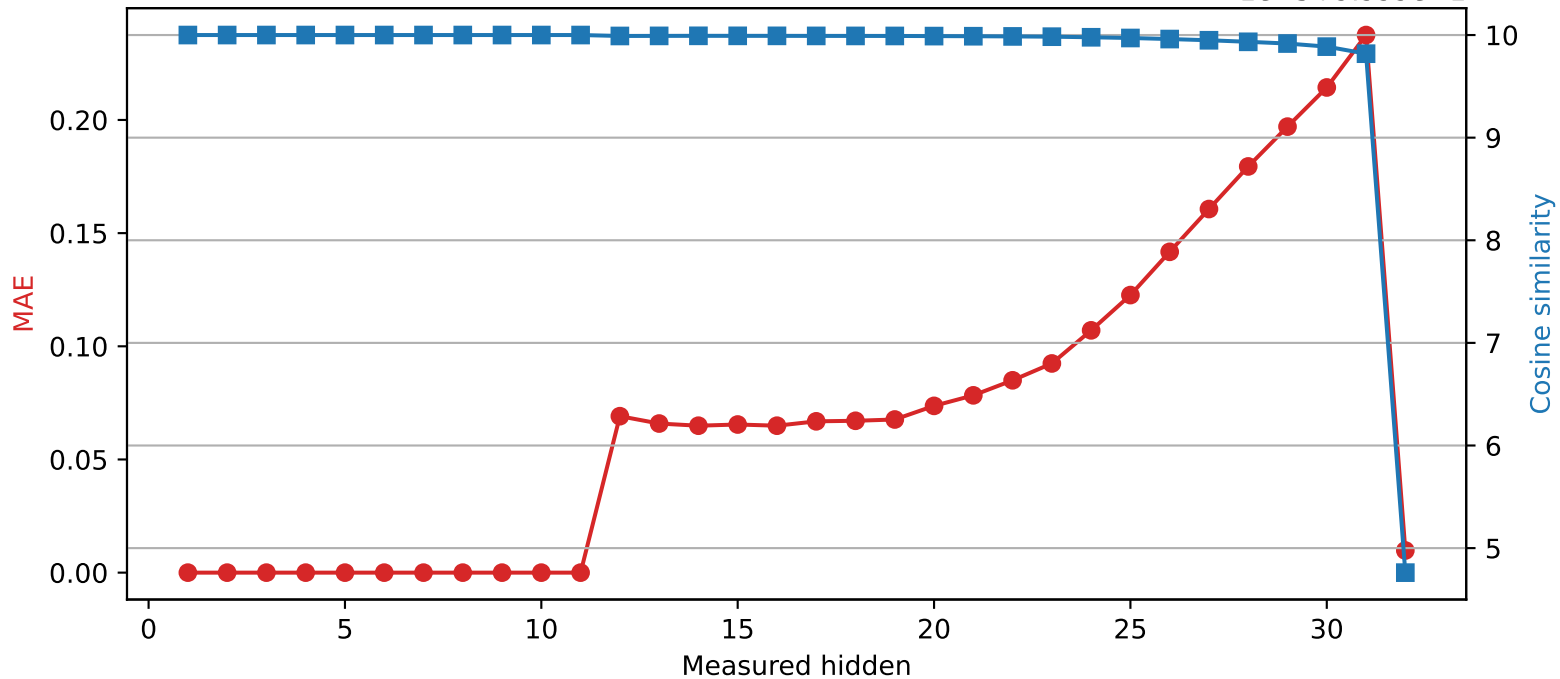
SmolLM2-360M | Quantized layer 11 | float16 \rightarrow int8 1e-5+9.999e-1
