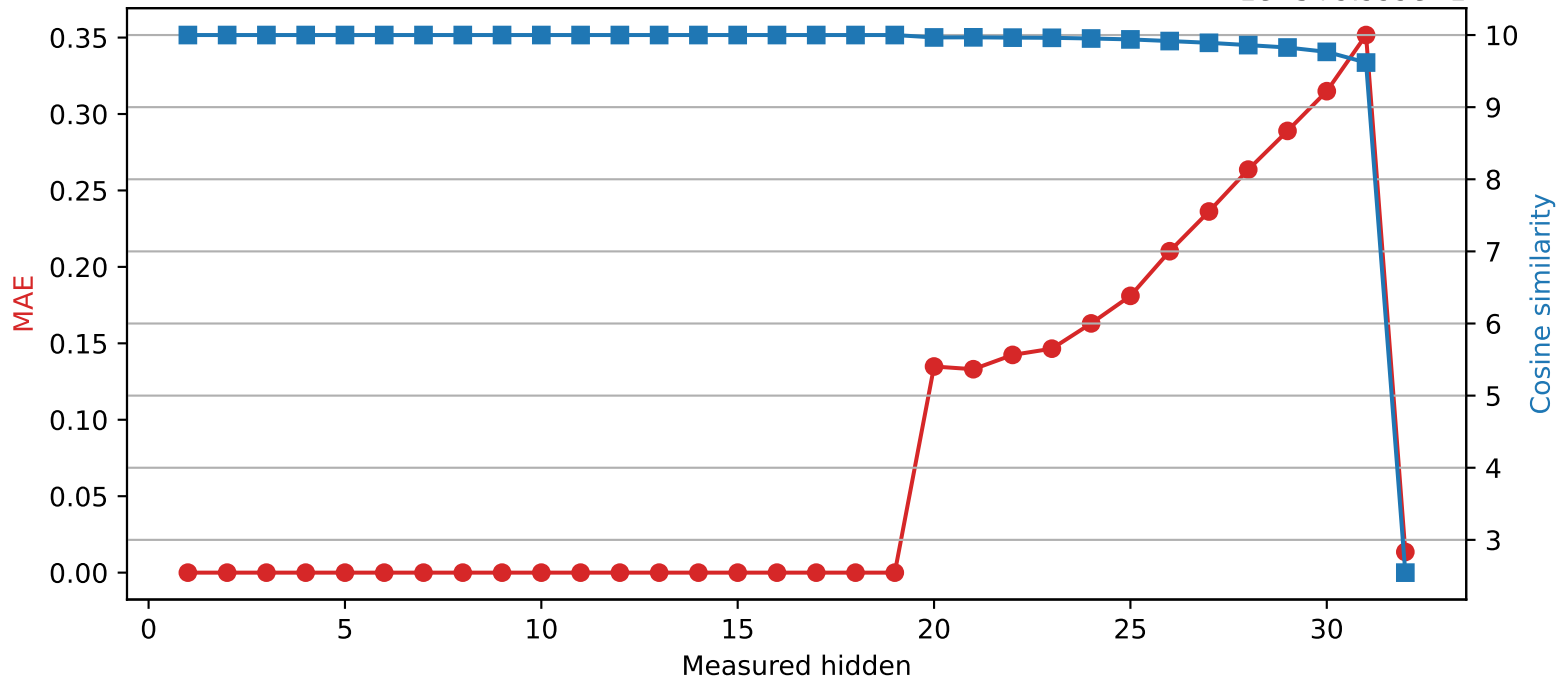
SmolLM2-360M | Quantized layer 19 | float16 → int8 1e-5 + 9.999e-1
