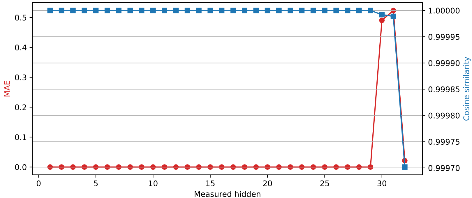
SmolLM2-360M | Quantized layer 29 | float16 \rightarrow int8
