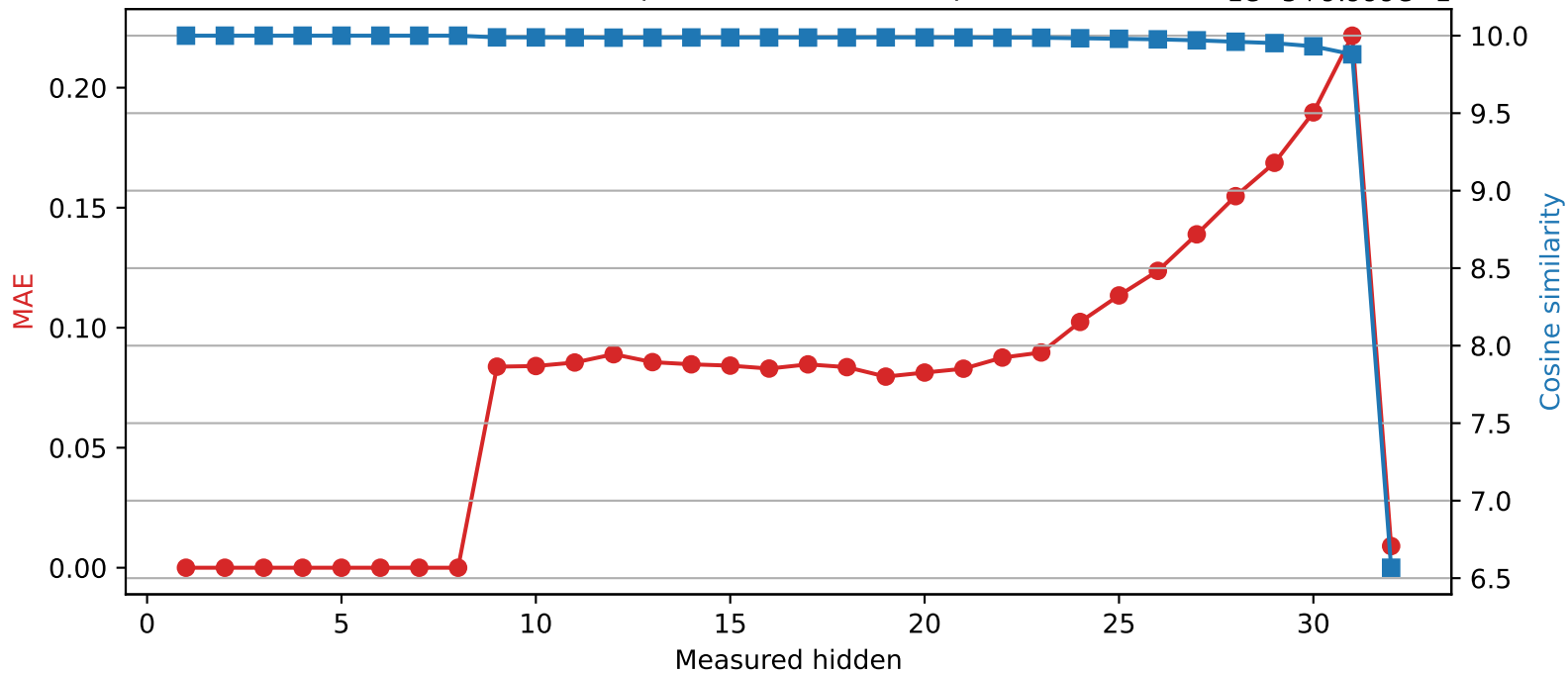
SmolLM2-360M | Quantized layer 8 | float16 → int8
