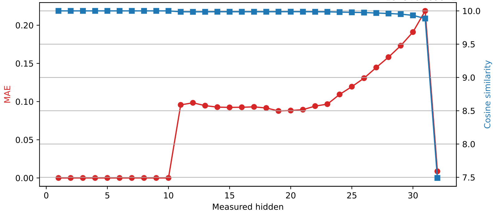
SmolLM2-360M | Quantized layer 10 | float16 → int8 1e-5+9.999e-1
