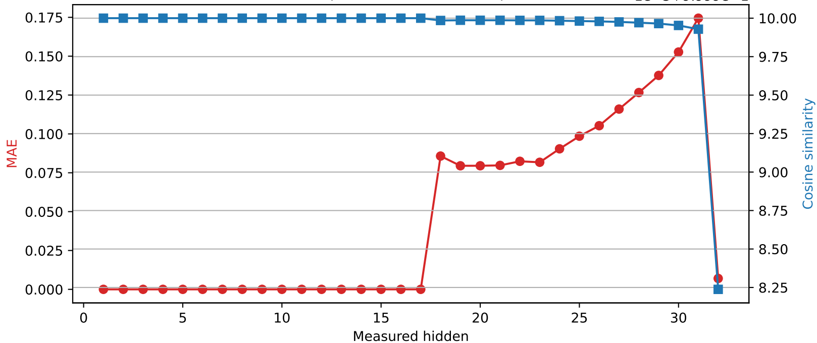
SmolLM2-360M | Quantized layer 17 | float16 \rightarrow int8 1e-5+9.999e-1
