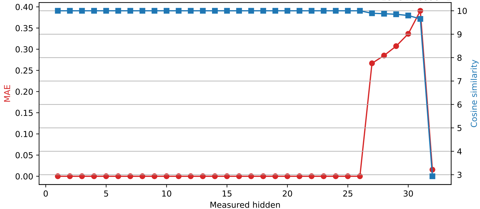
SmolLM2-360M | Quantized layer 26 | float16 → int8 1e-5+9.999e-1
