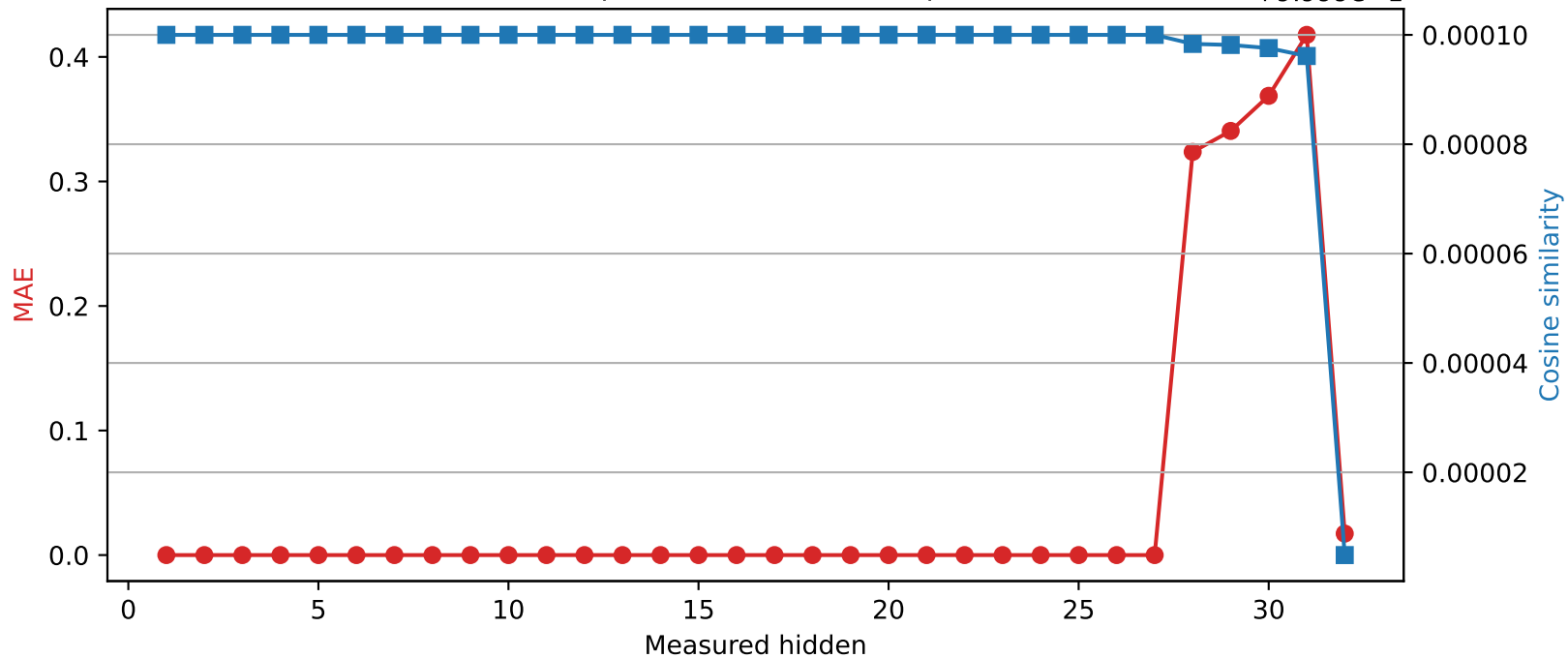
SmolLM2-360M | Quantized layer 27 | float16 → int8
