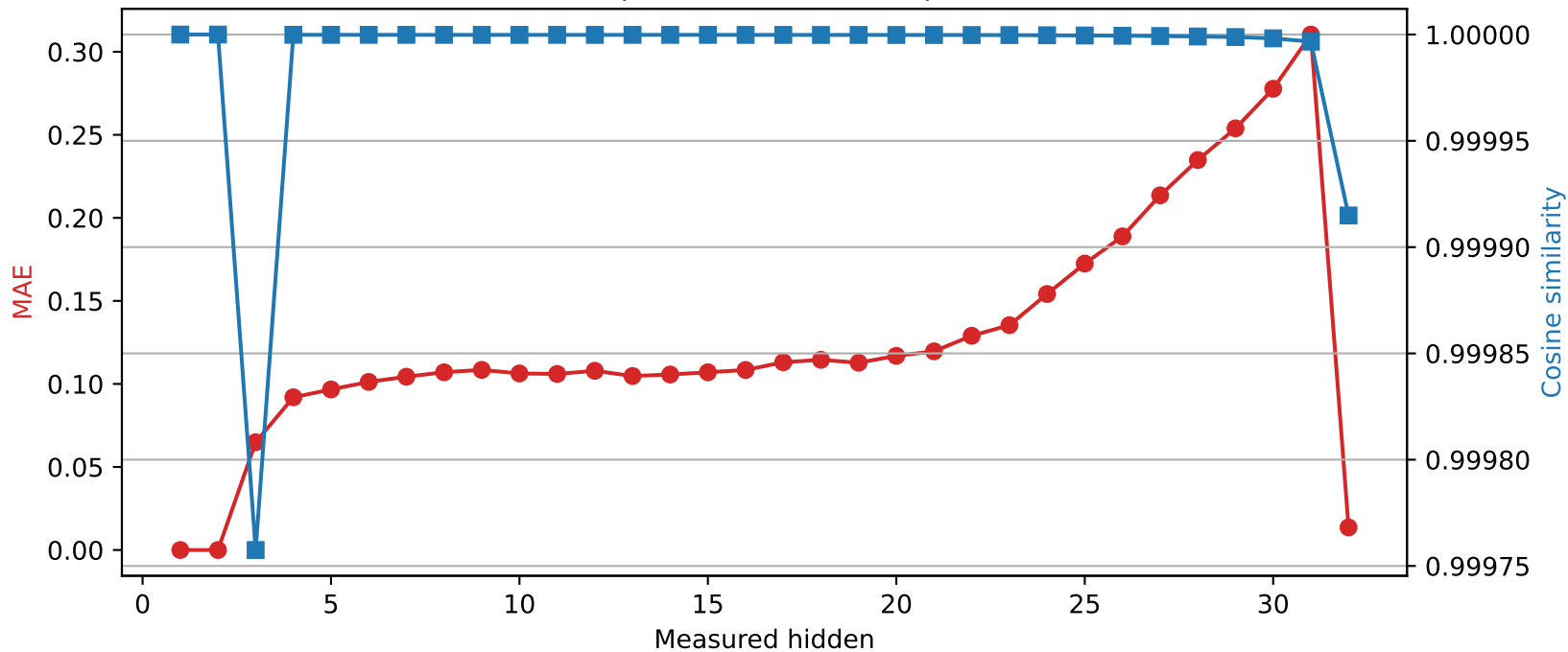
SmolLM2-360M | Quantized layer 2 | float16 → int8
