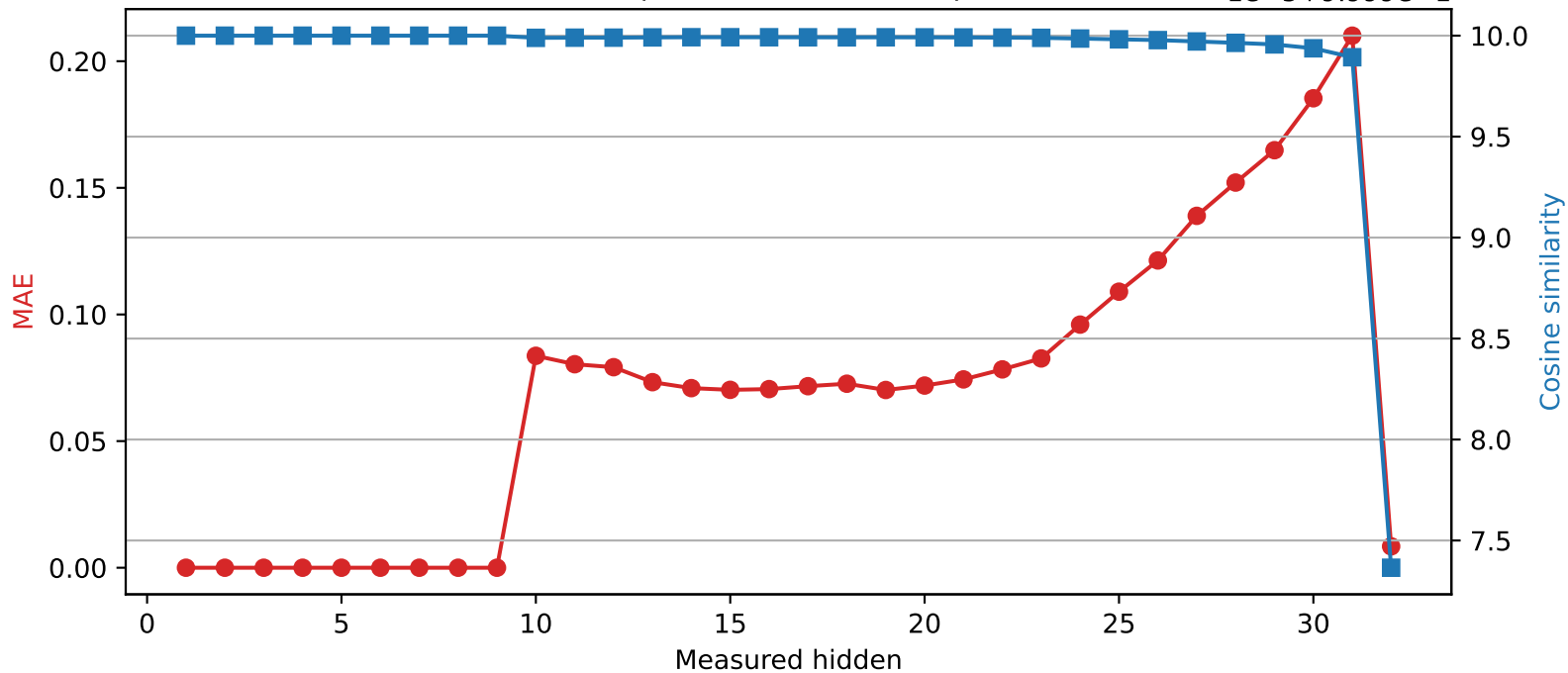
SmolLM2-360M | Quantized layer 9 | float16 → int8
