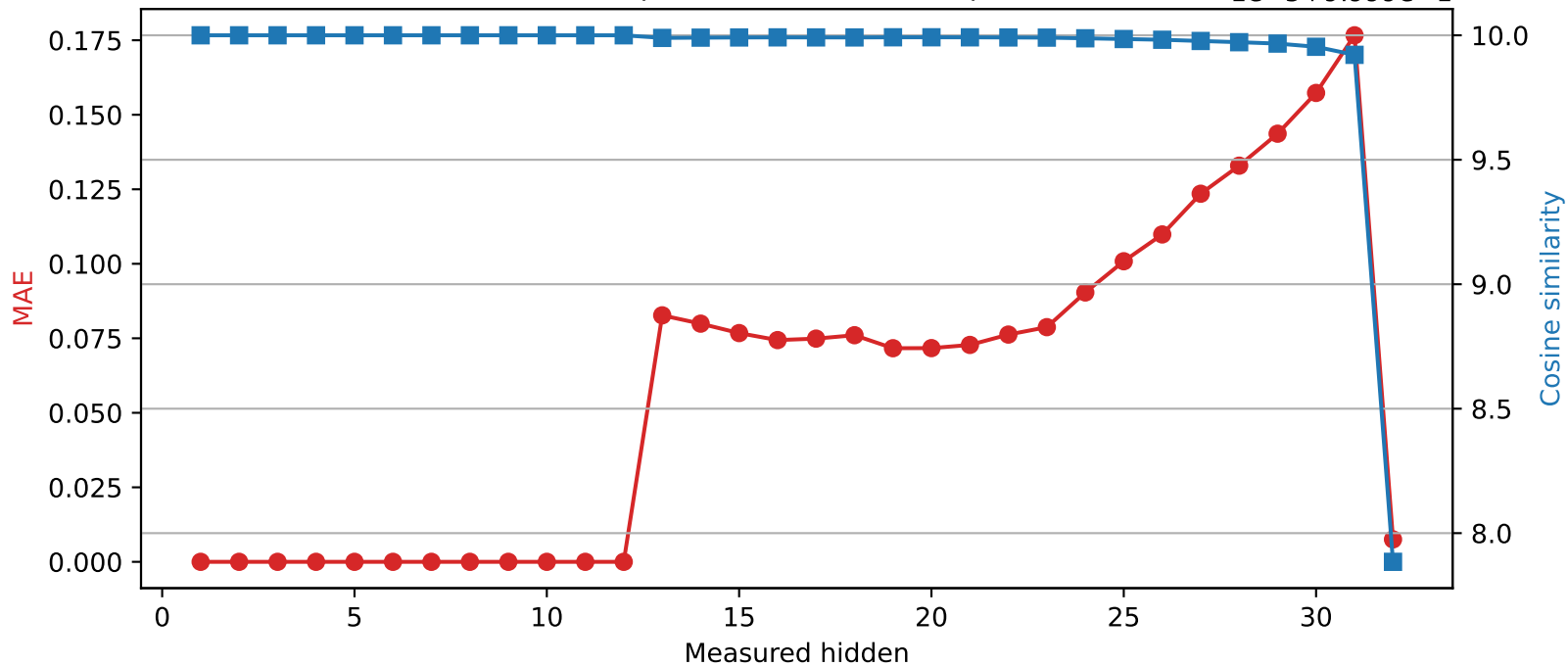
SmolLM2-360M | Quantized layer 12 | float16 → int8 1e-5 + 9.999e-1
