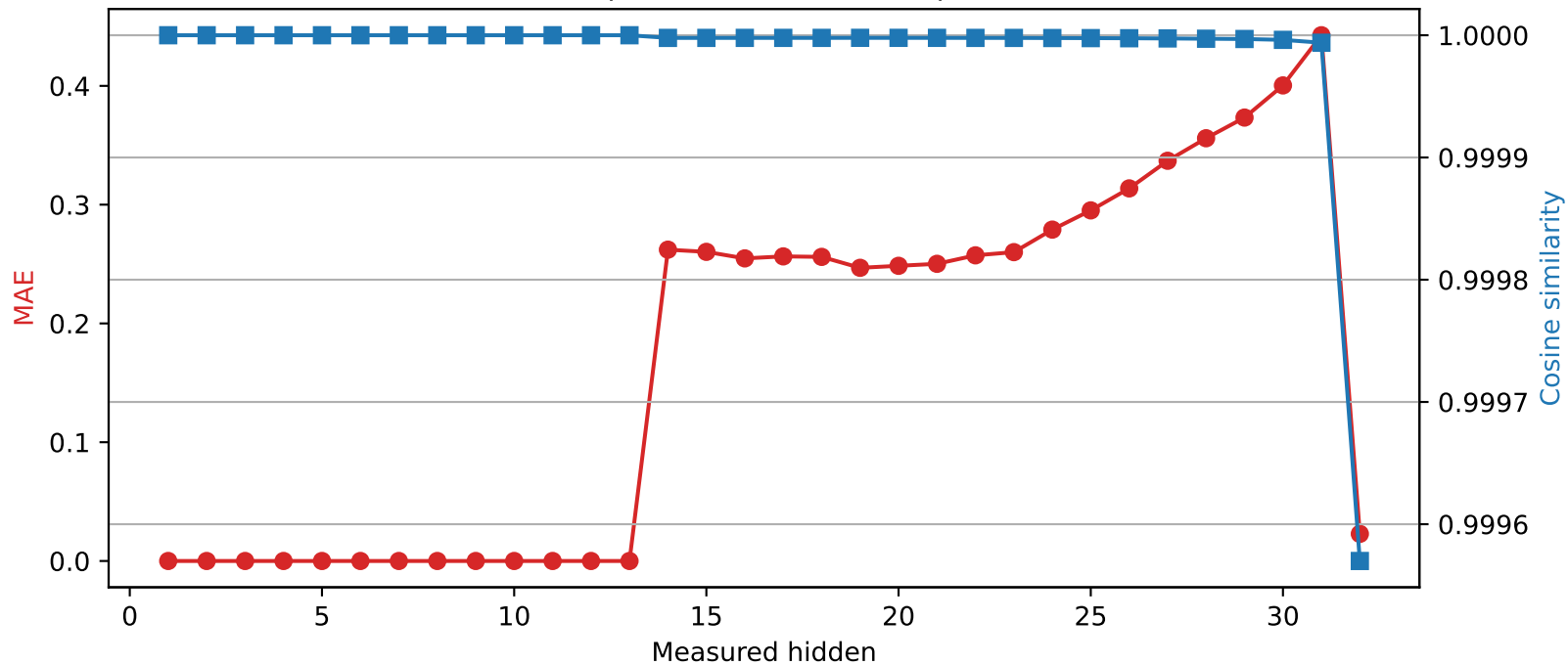
SmolLM2-360M | Quantized layer 13 | float16 → int8
