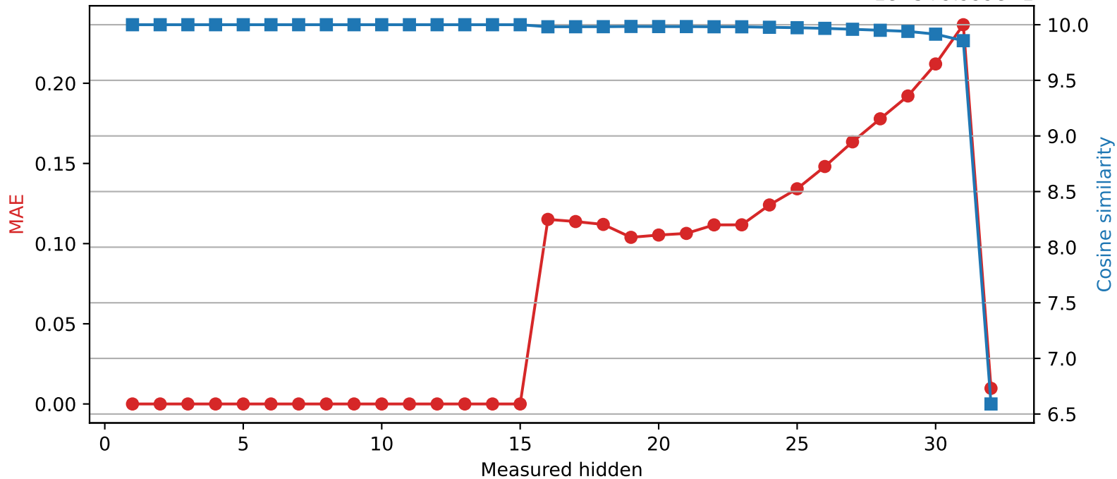
SmolLM2-360M | Quantized layer 15 | float16 → int8 1e-5 + 9.999e-1
