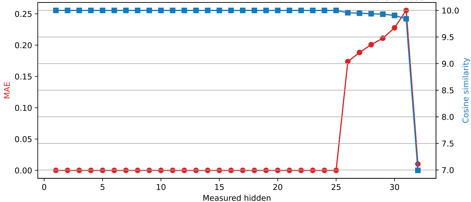
SmolLM2-360M | Quantized layer 25 | float16 → int8 1e-5 + 9.999e-1
