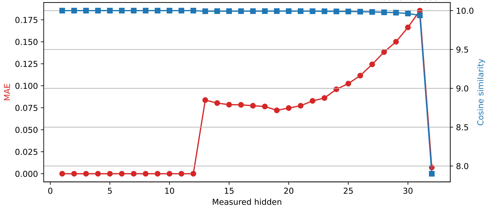
SmolLM2-360M | Quantized layer 12 | float16 \rightarrow int8 1e-5+9.999e-1
