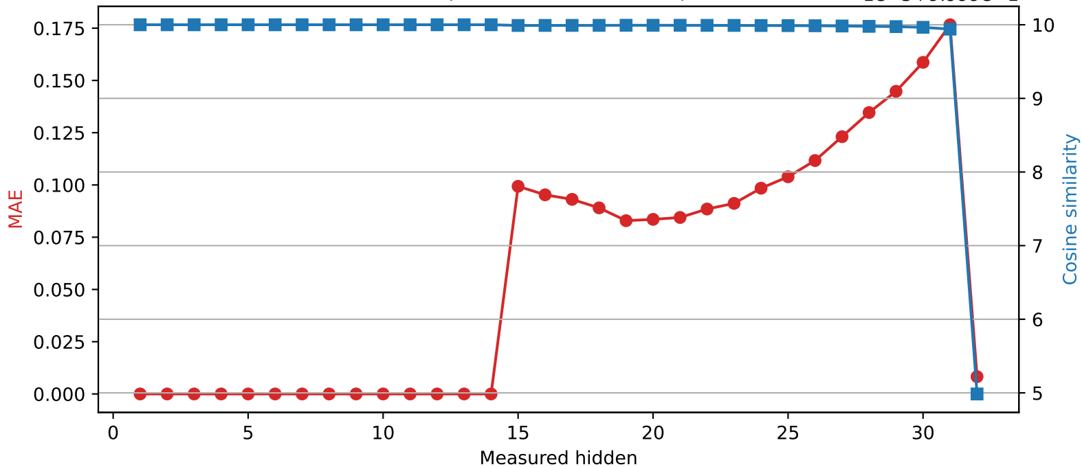
SmolLM2-360M | Quantized layer 14 | float16 \rightarrow int8 1e-5+9.999e-1
