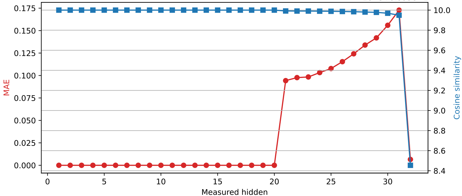
SmolLM2-360M | Quantized layer 20 | float16 → int8 1e-5+9.999e-1
