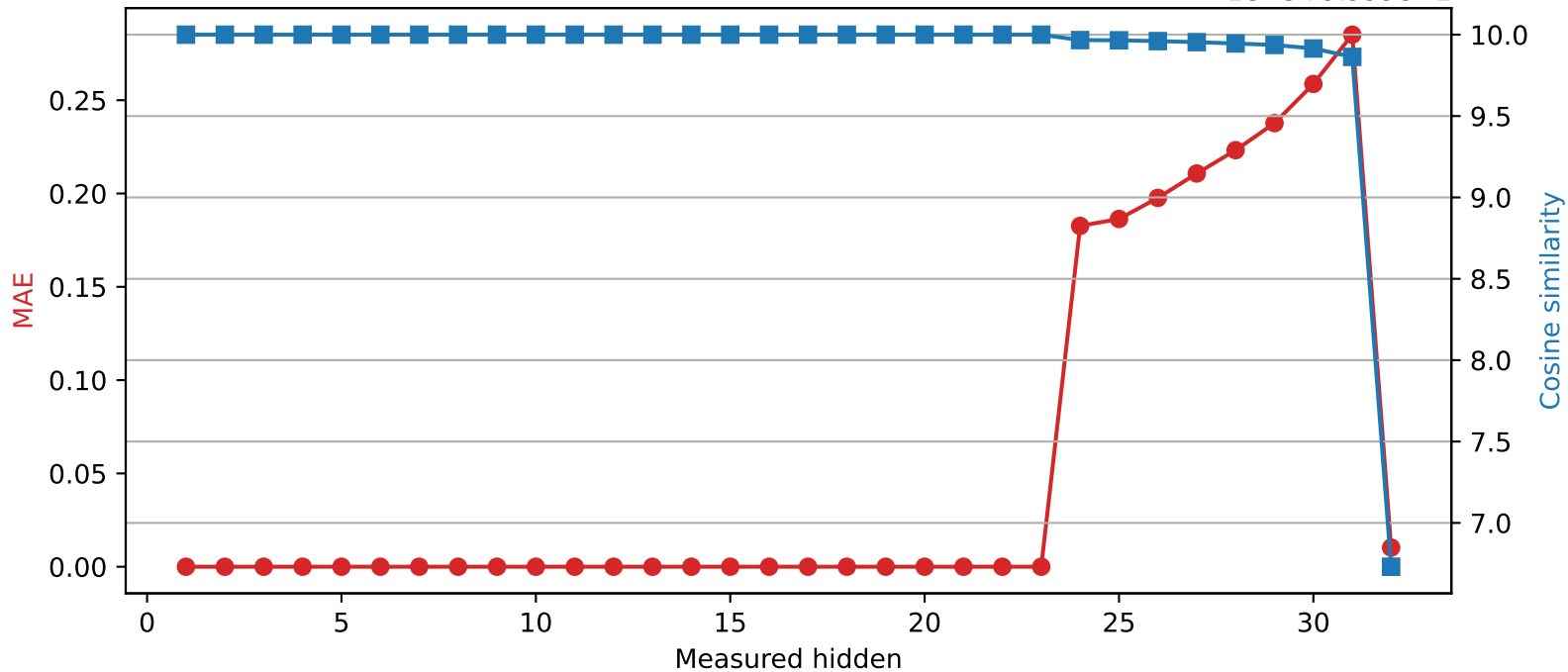
SmolLM2-360M | Quantized layer 23 | float16 → int8 1e-5 + 9.999e-1
