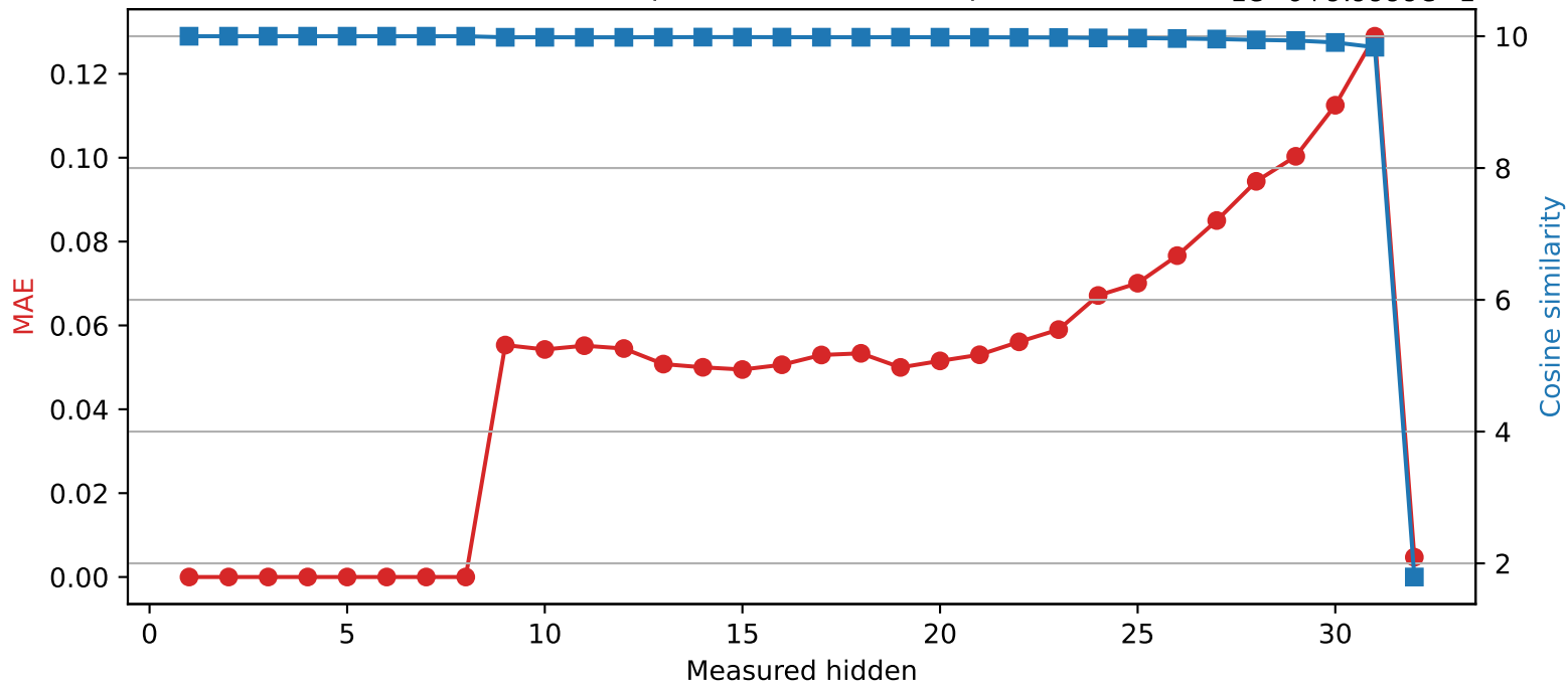
SmolLM2-360M | Quantized layer 8 | float32 \rightarrow int8 1e-6+9.9999e-1
