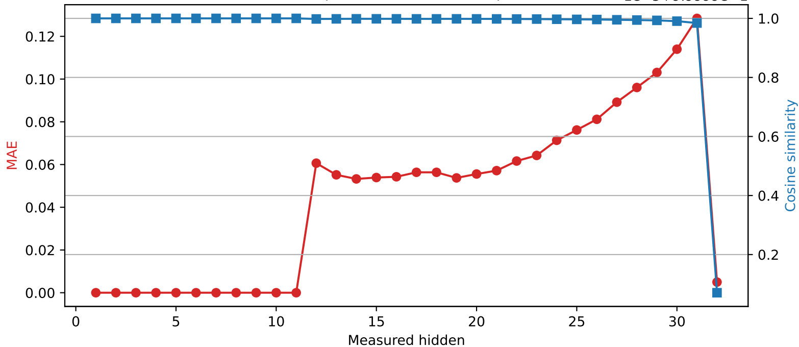
SmolLM2-360M | Quantized layer 11 | float32 \rightarrow int8 1e-5+9.9999e-1
