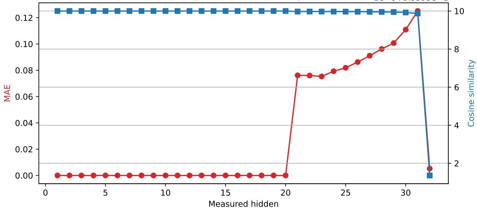
SmolLM2-360M | Quantized layer 20 | float32 \rightarrow int8 1e-6+9.9999e-1
