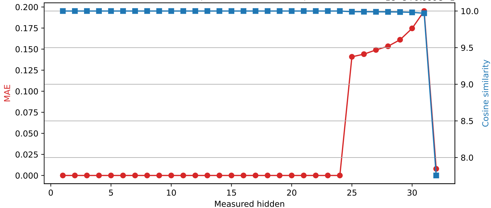
SmolLM2-360M | Quantized layer 24 | float32 → int8 1e-5+9.999e-1
