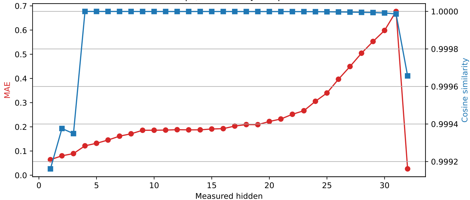
SmolLM2-360M | Quantized layer 0 | float32 → int8
