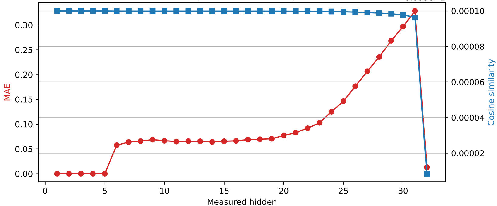
SmolLM2-360M | Quantized layer 5 | float32 \rightarrow int8
