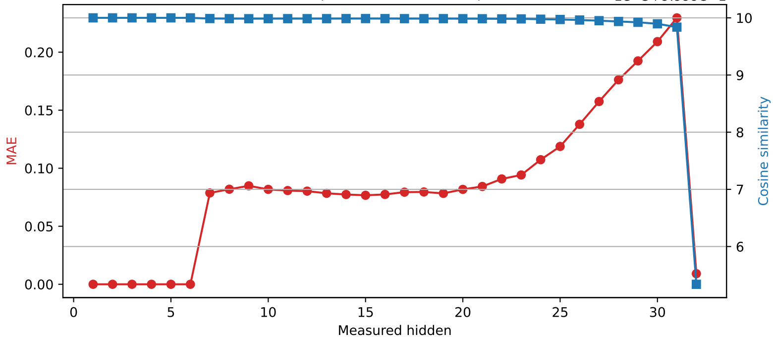
SmolLM2-360M | Quantized layer 6 | float32 → int8
