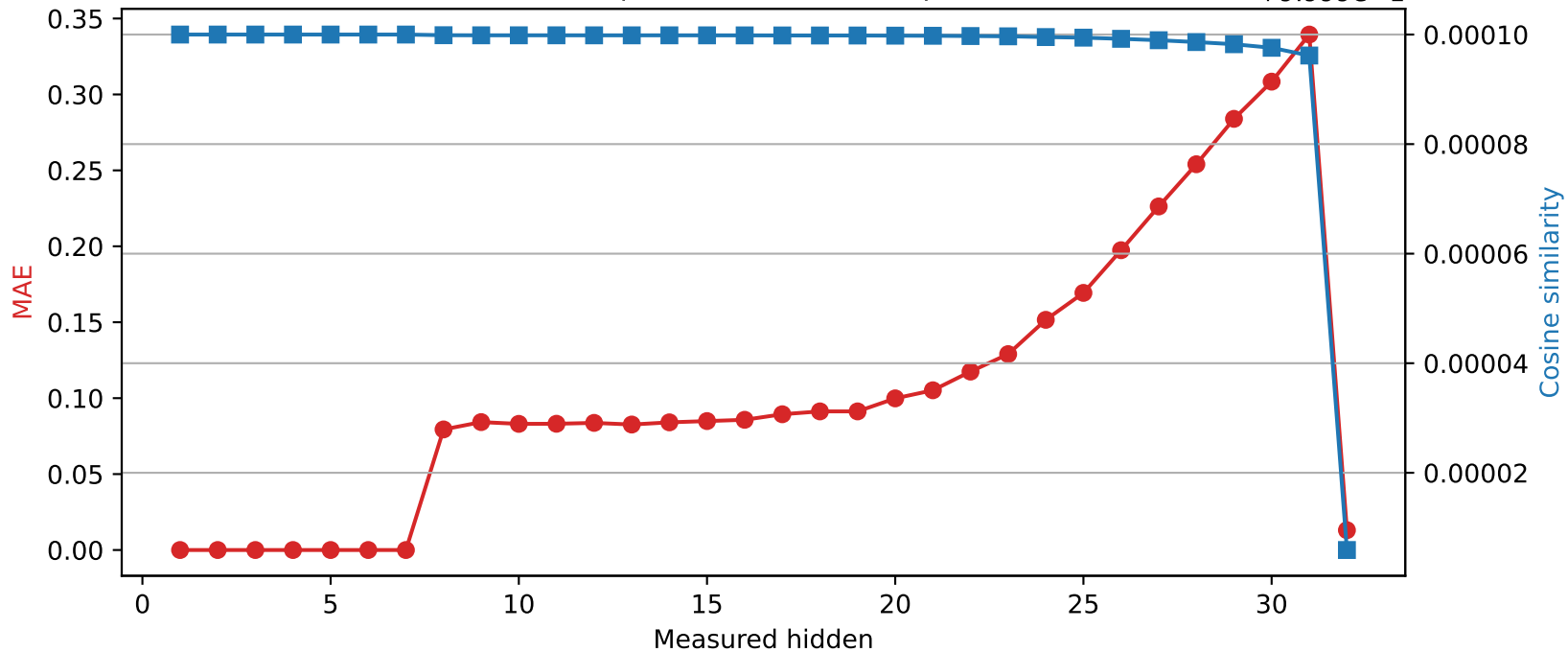
SmolLM2-360M | Quantized layer 7 | float32 → int8
