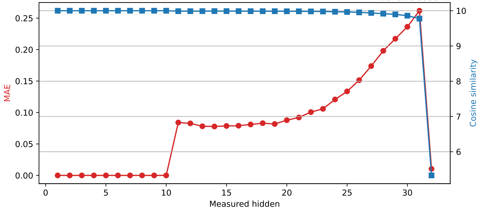
SmolLM2-360M | Quantized layer 10 | float32 \rightarrow int8 1e-5+9.999e-1
