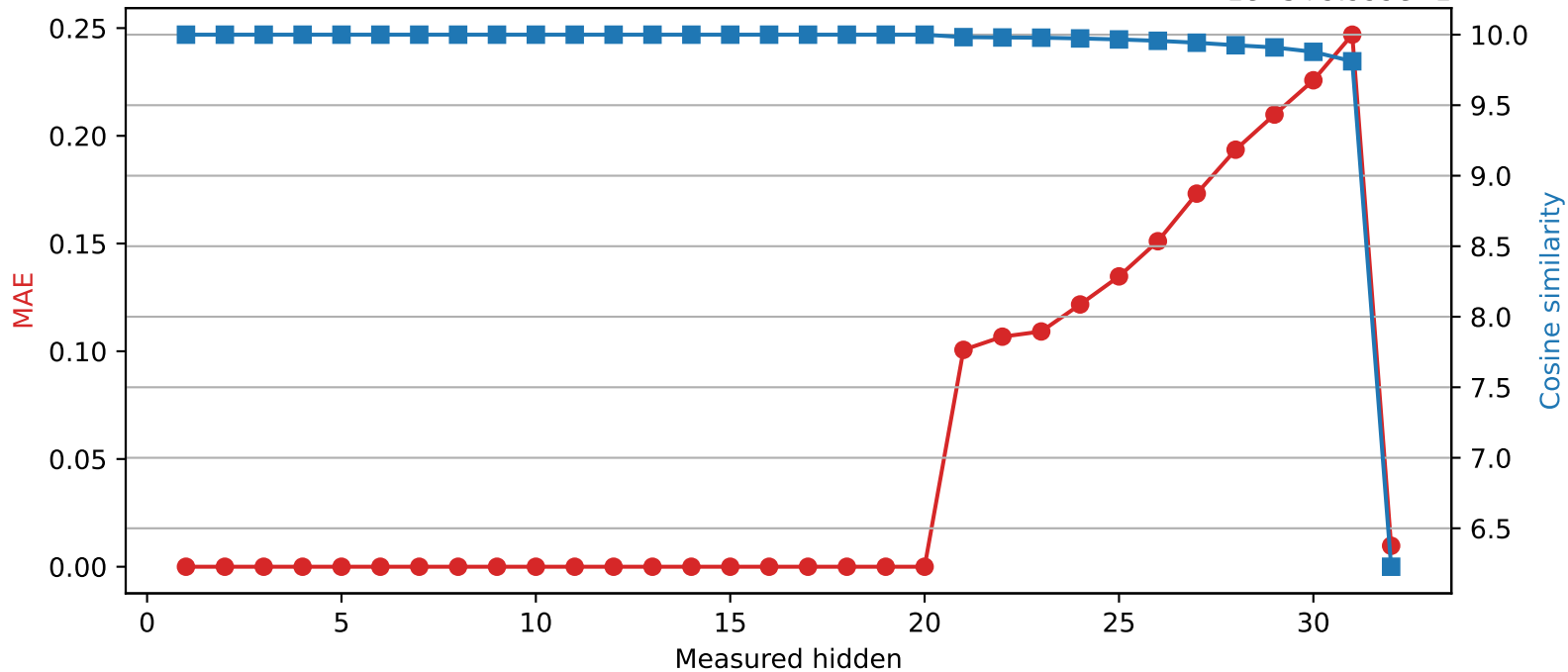
SmolLM2-360M | Quantized layer 20 | float32 → int8 1e-5+9.999e-1
