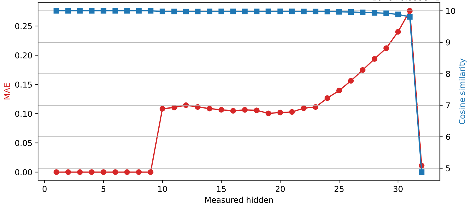
SmolLM2-360M | Quantized layer 9 | float32 → int8
