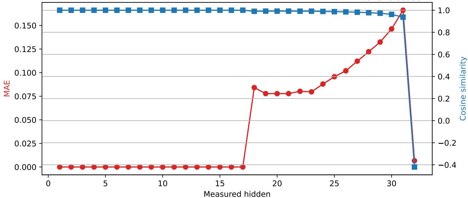
SmolLM2-360M | Quantized layer 17 | float32 → int8 1e-5 + 9.9999e-1
