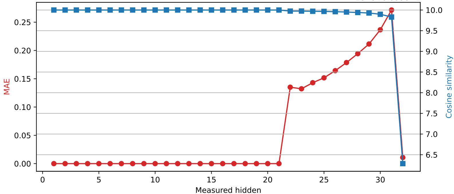
SmolLM2-360M | Quantized layer 21 | float32 → int8 1e-5 + 9.999e-1
