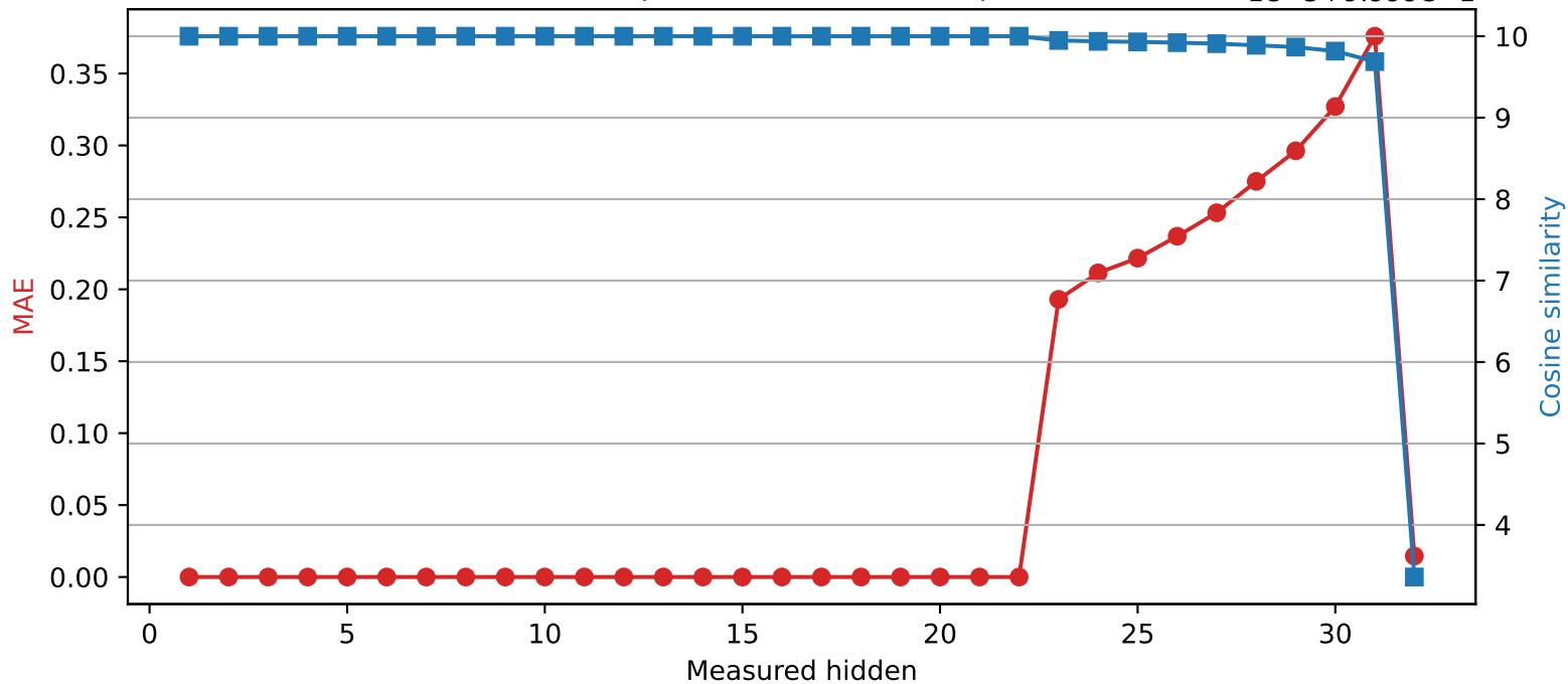
SmolLM2-360M | Quantized layer 22 | float32 \rightarrow int8 1e-5+9.999e-1
