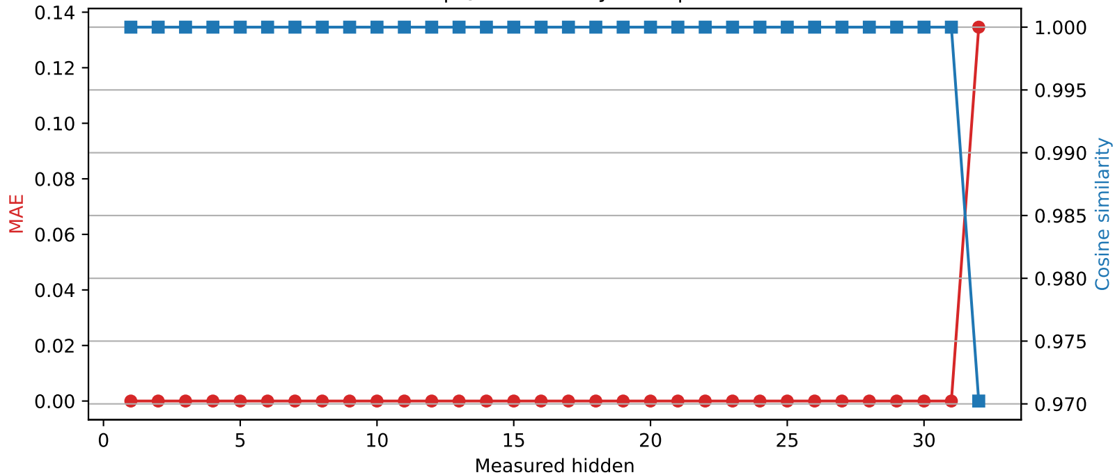
SmolLM2-360M | Quantized layer 31 | float32 → int8
