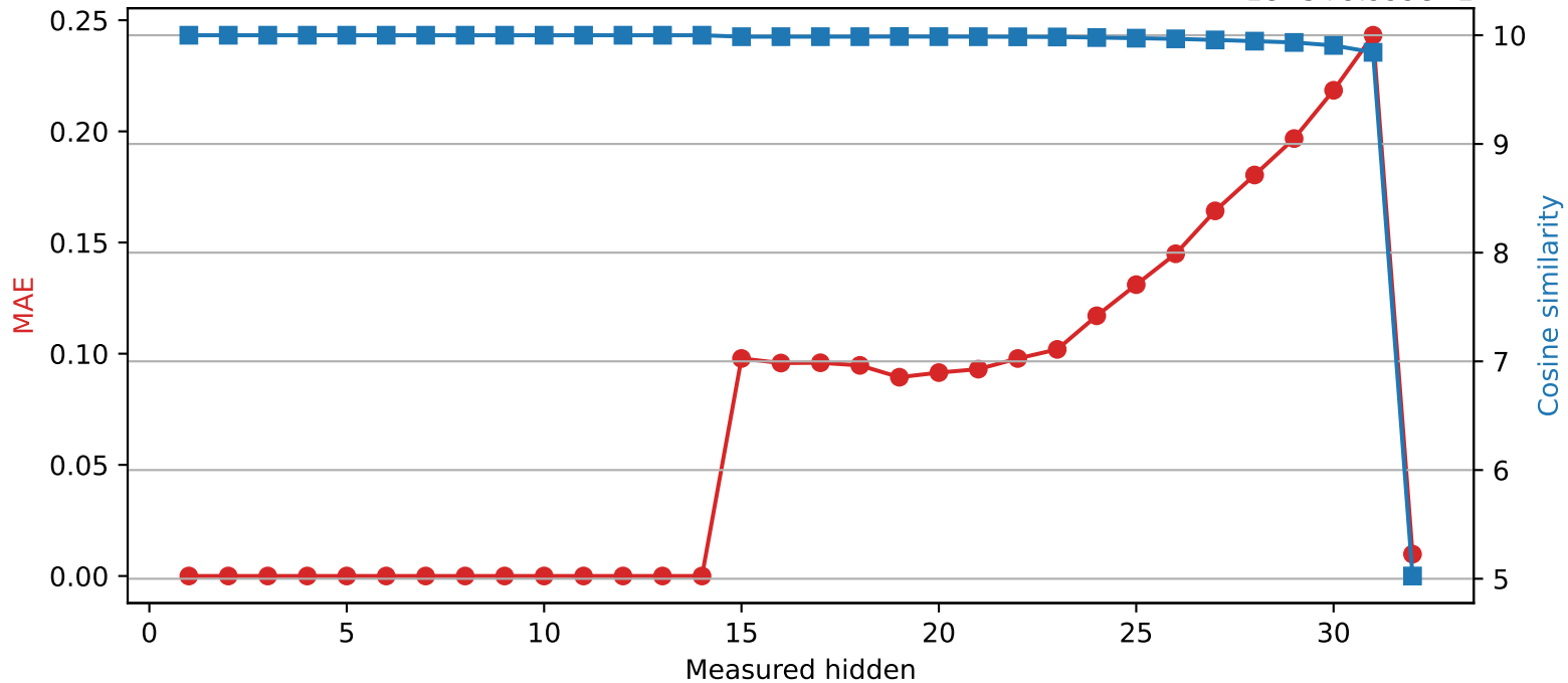
SmolLM2-360M | Quantized layer 14 | float32 \rightarrow int8 1e-5+9.999e-1
