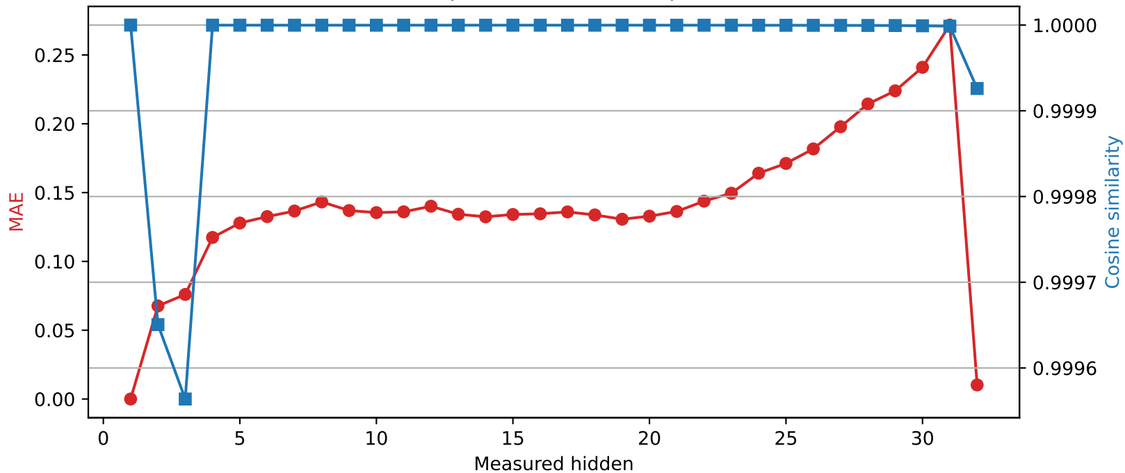
SmolLM2-360M | Quantized layer 1 | float32 \rightarrow int8
