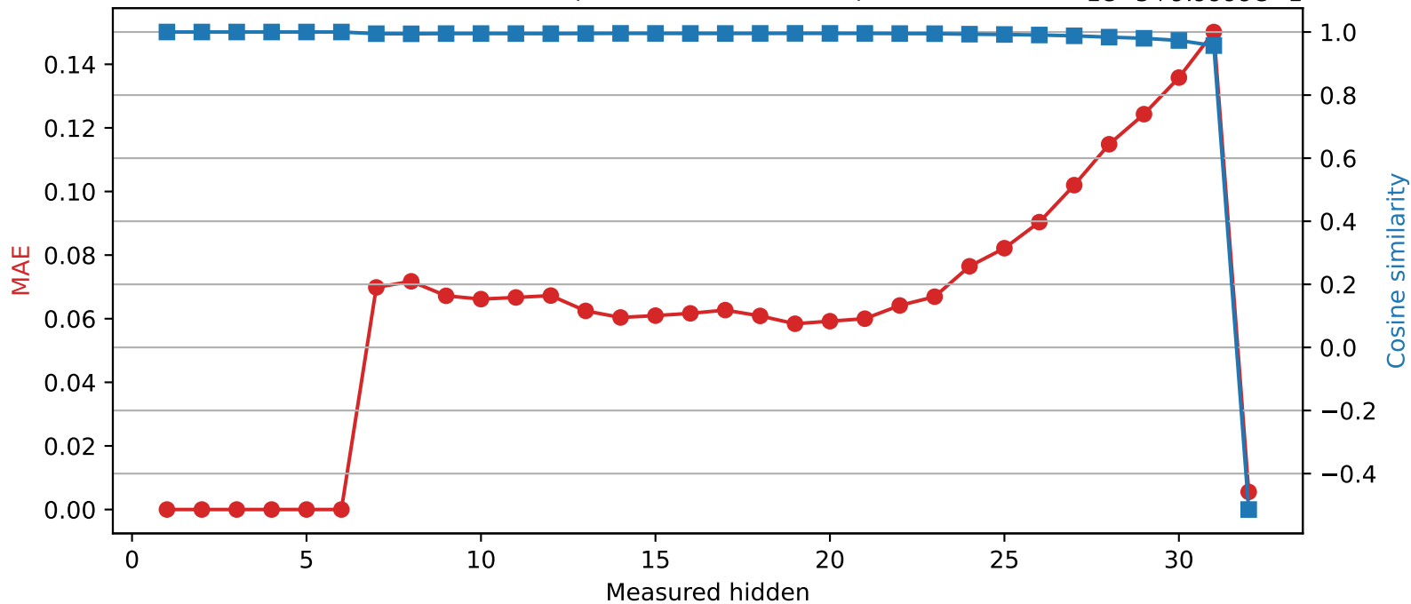
SmolLM2-360M | Quantized layer 6 | float32 → int8 1e-5+9.9999e-1
