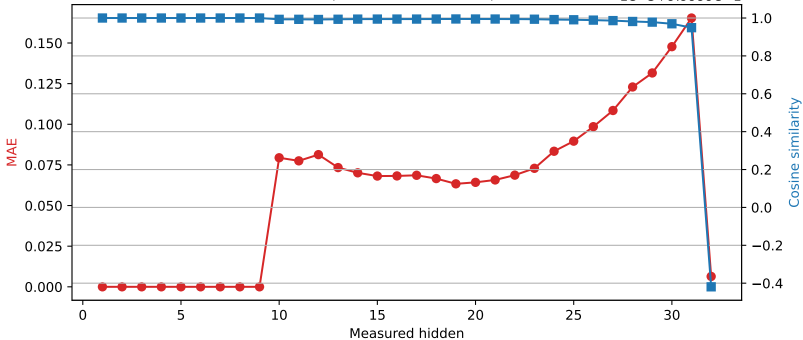
SmolLM2-360M | Quantized layer 9 | float32 → int8 1e-5 + 9.9999e-1
