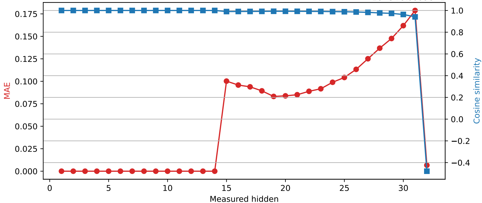
SmolLM2-360M | Quantized layer 14 | float32 \rightarrow int8 1e-5+9.9999e-1
