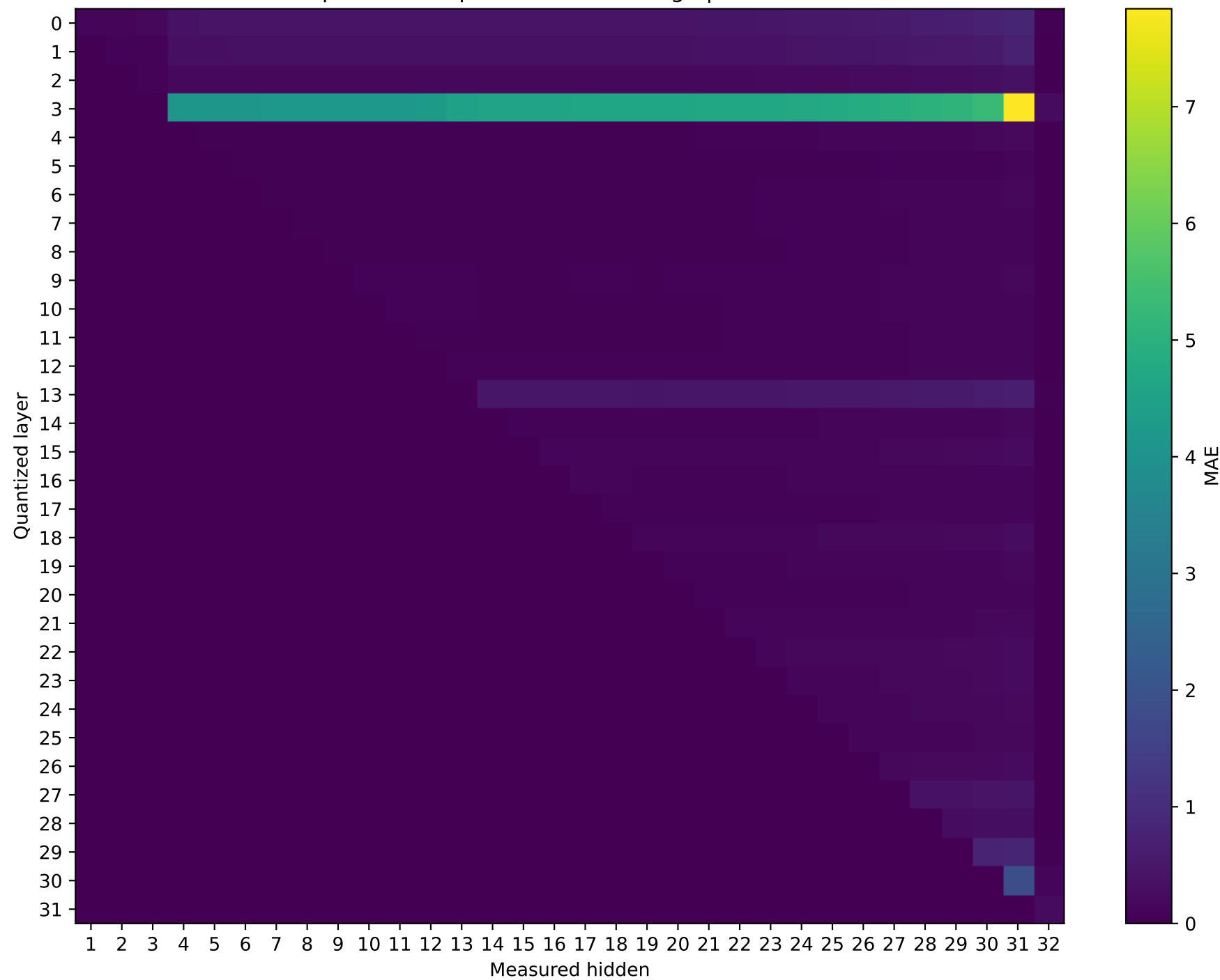
SmolLM2-360M Prompt 0: MAE representation damage | float64 → int8
