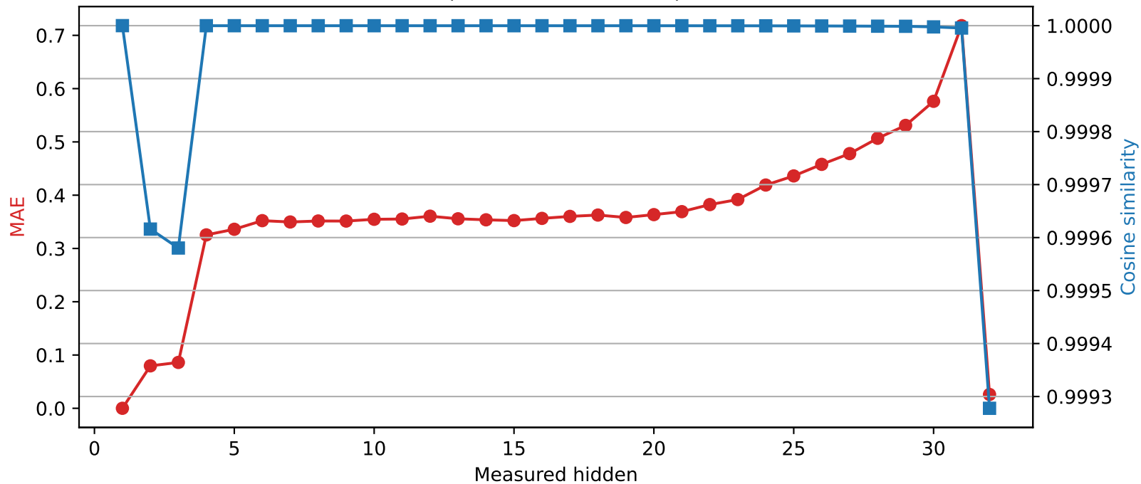
SmolLM2-360M | Quantized layer 1 | float64 → int8
