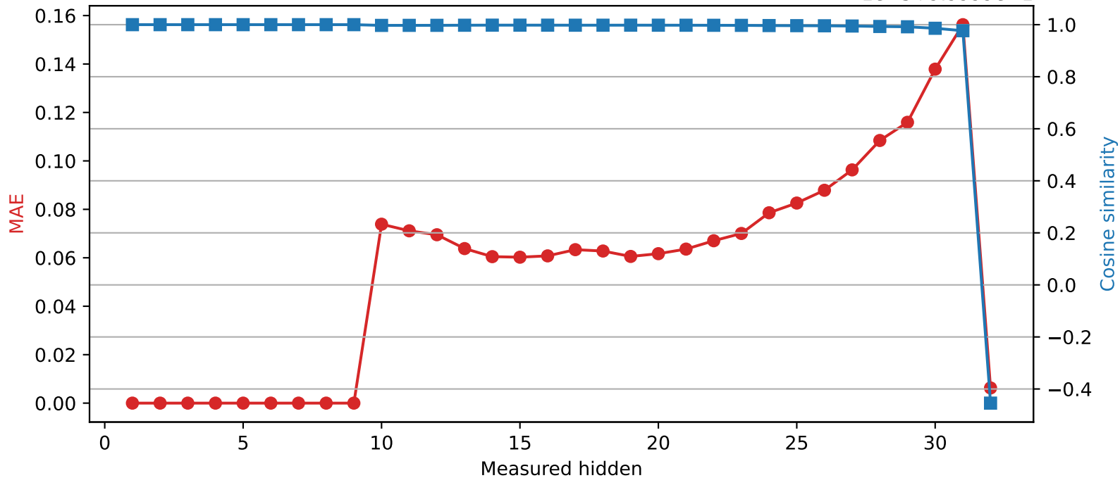
SmolLM2-360M | Quantized layer 9 | float64 → int8 1e-5+9.9999e-1
