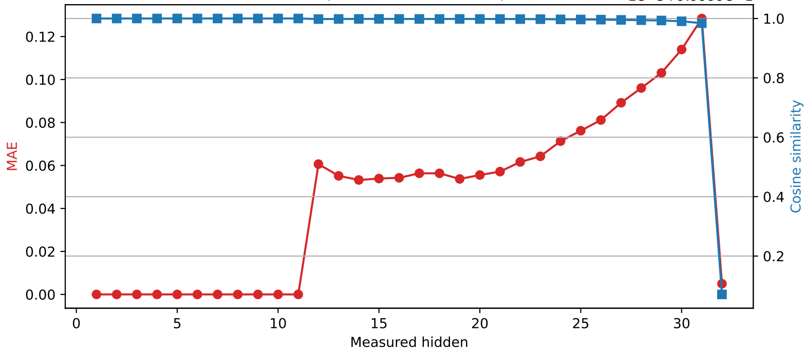
SmolLM2-360M | Quantized layer 11 | float64 \rightarrow int8 1e-5+9.9999e-1
