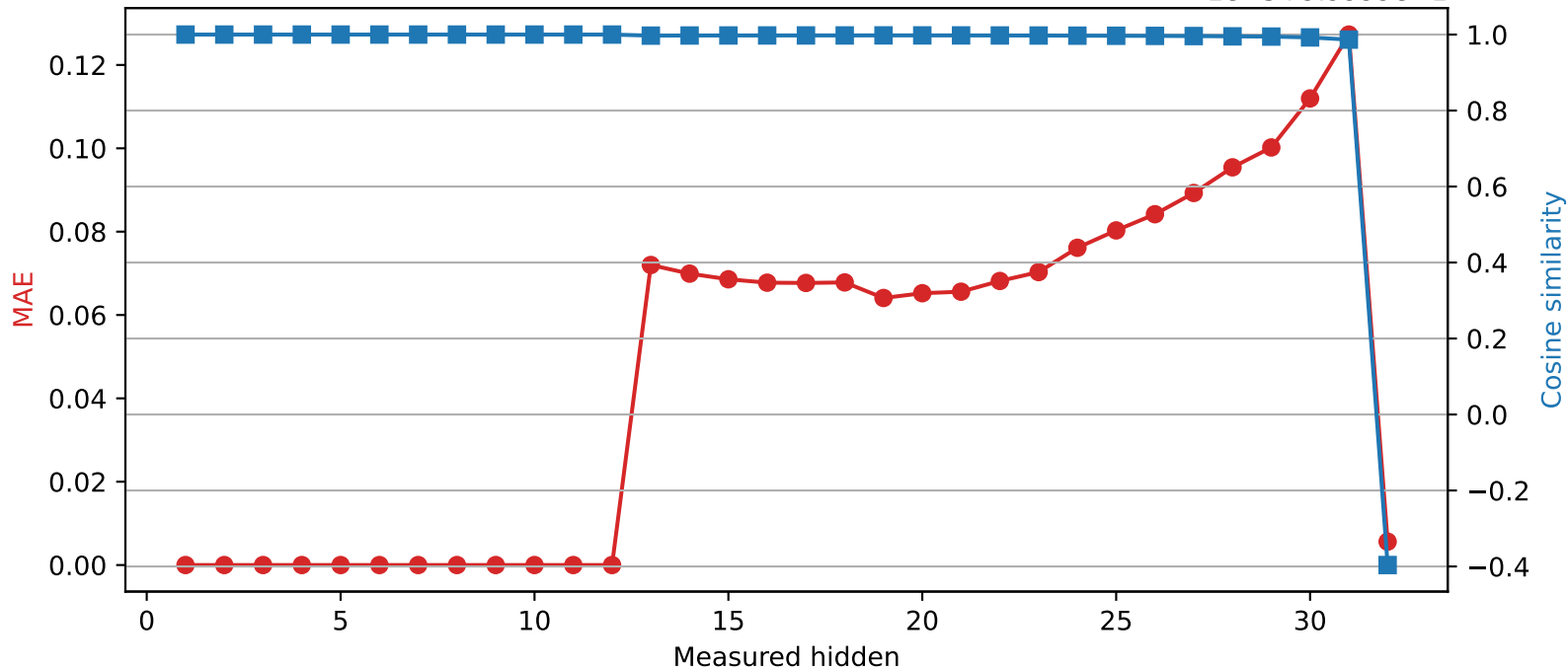
SmolLM2-360M | Quantized layer 12 | float64 → int8 1e-5 + 9.9999e-1
