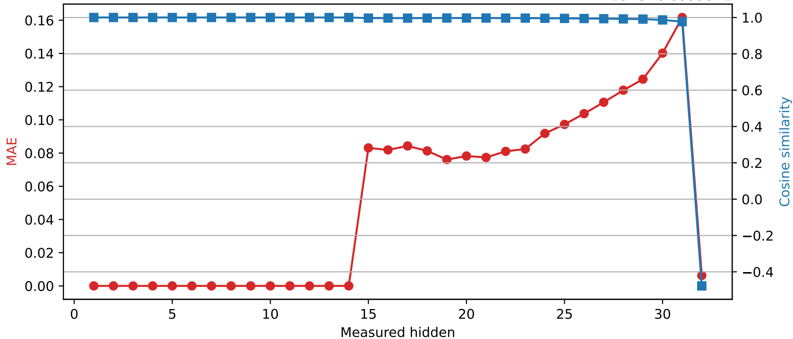
SmolLM2-360M | Quantized layer 14 | float64 \rightarrow int8 1e-5+9.9999e-1
